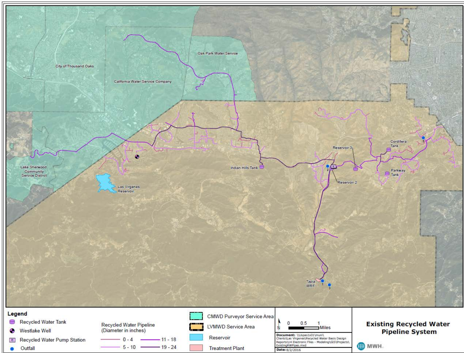
Figure 2-5 Recycled Water System
